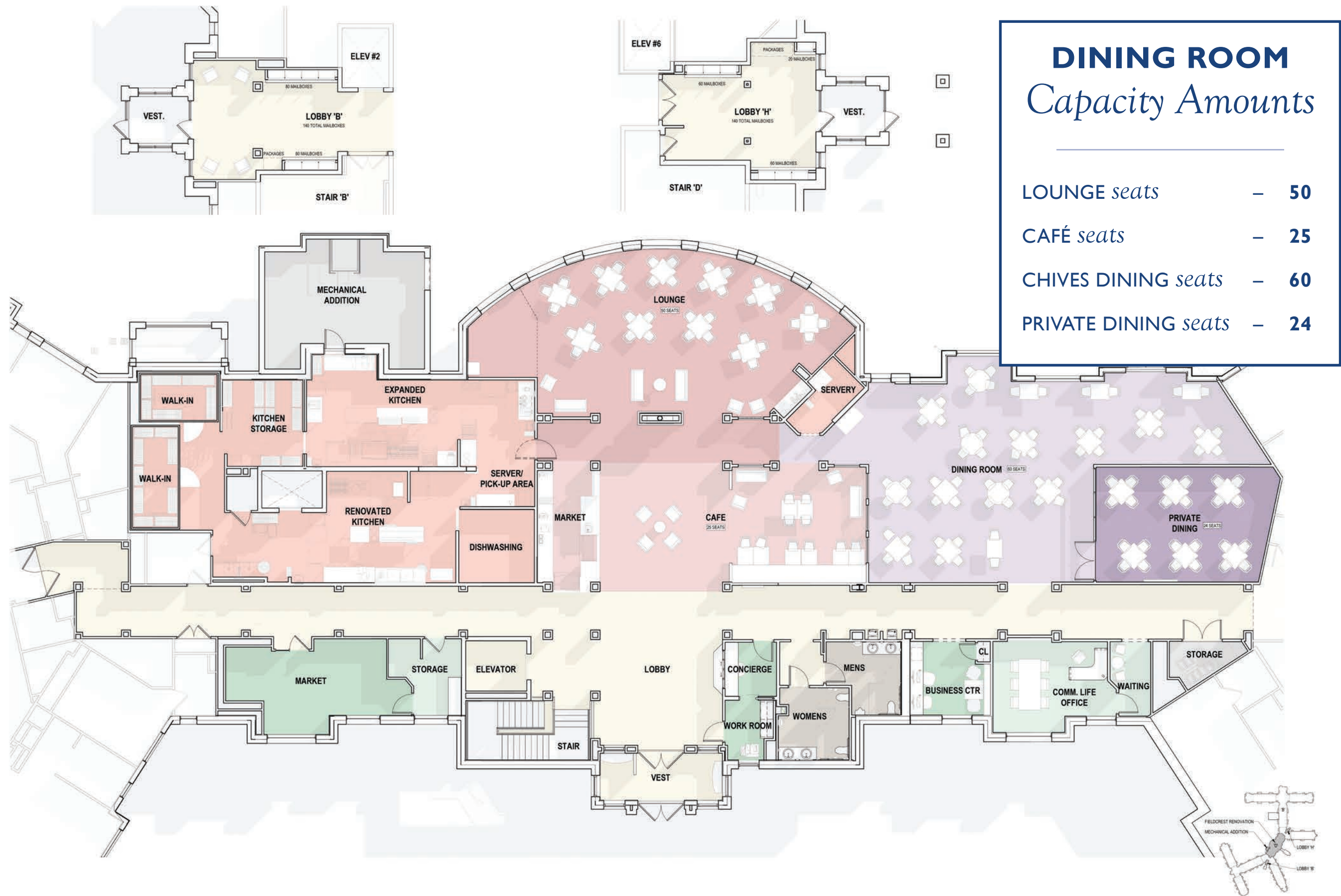
FIELDCREST - FIRST FLOOR PLAN FIELDCREST RENOVATIONS AND ADDITIONS BRETHREN VILLAGE 01/31/2023
